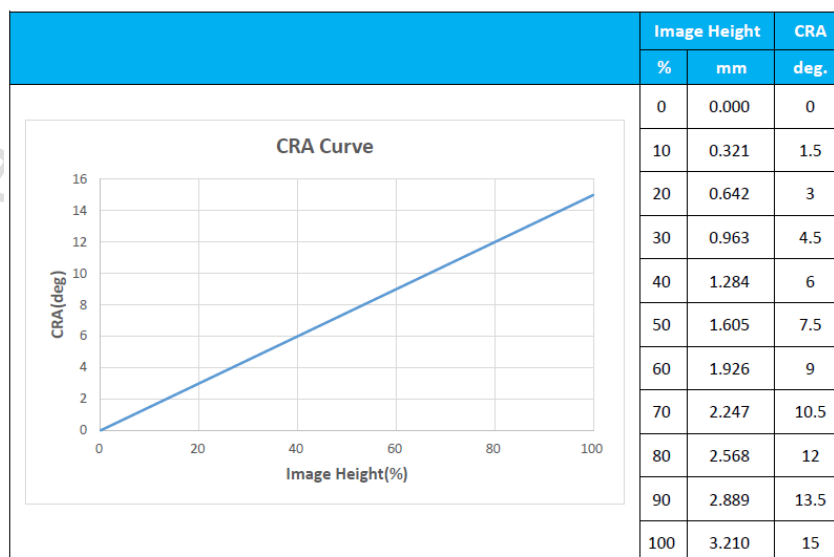
图 4-2 CRA Curve
